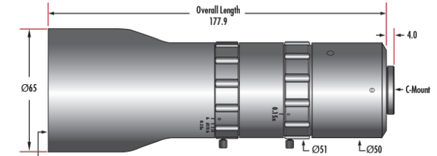
0.25X - 0.5X Telecentric VariMagTL® Lens (#88-385)
