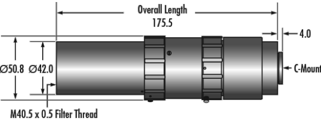
0.5X - 1.0X Telecentric VariMagTL® Lens (#88-386)
