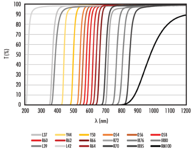
Hoya Colored Glass Longpass Filters
