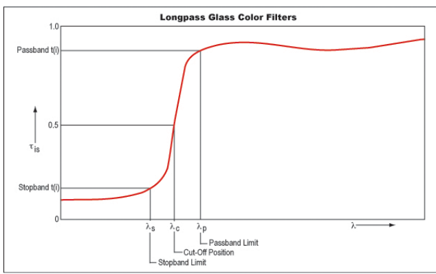
Hoya Colored Glass Longpass Filters
