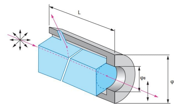
Glan-Laser Polarizers
