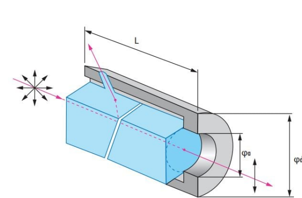
Glan-Laser Polarizers
