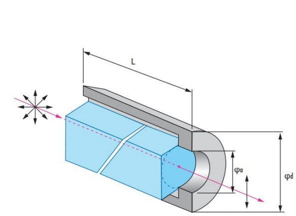
Glan-Taylor Polarizers
