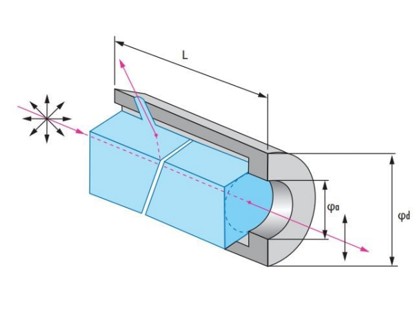
Glan-Laser Polarizers
