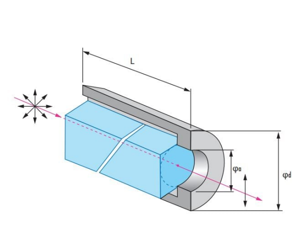
Glan-Taylor Polarizers
