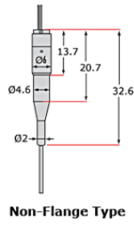
Non-Flange Type
