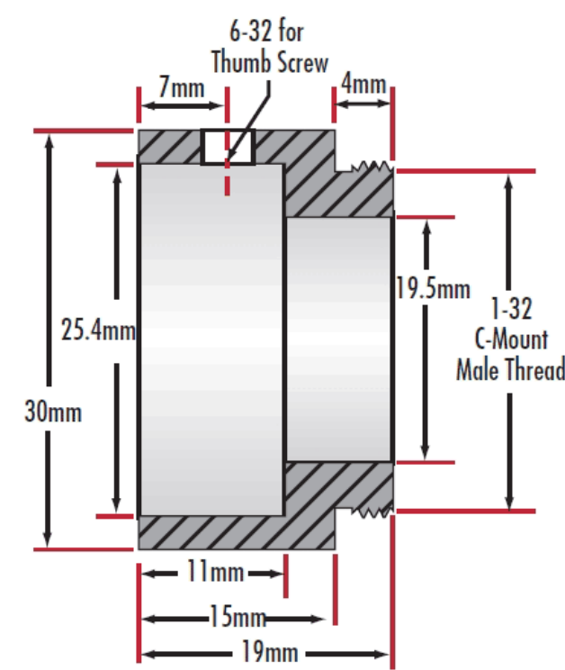
C-Mount Dimensions
