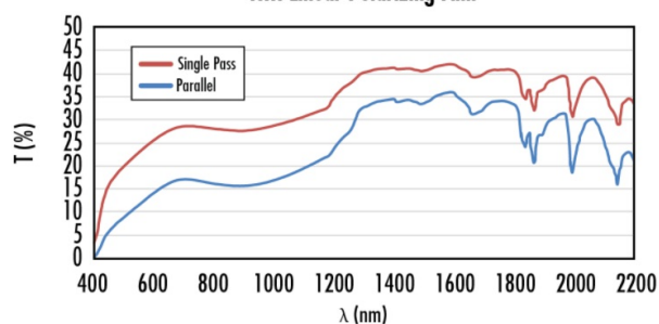
NIR Linear Polarizing Film
