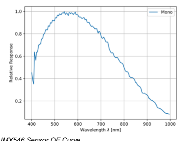
IMX546 Sensor QE Curve
