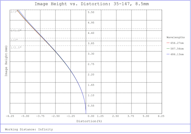
#35-147, 8.5mm, f/1.8, 75mm-∞ Primary WD, HRr Series Fixed Focal Length Lens, Distortion Plot
