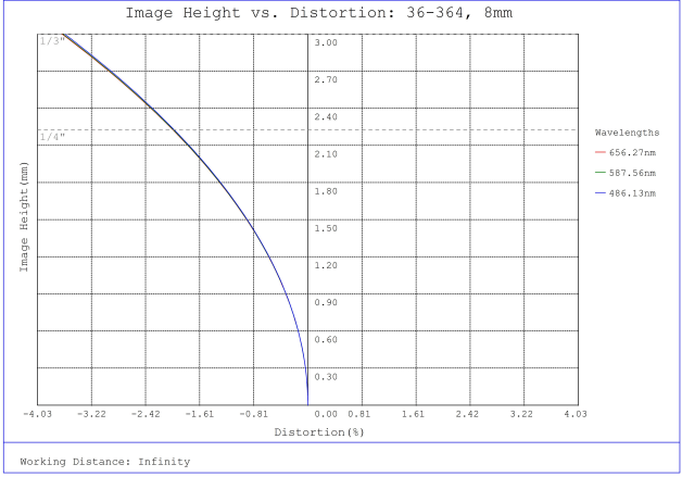
#36-364, 8.0mm FL f/2.5, Rugged Blue Series M12 Lens, Distortion Plot
