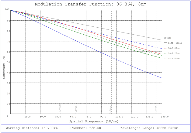
#36-364, 8.0mm FL f/2.5, Rugged Blue Series M12 Lens, Modulated Transfer Function (MTF) Plot, 150mm Working Distance, f2.5
