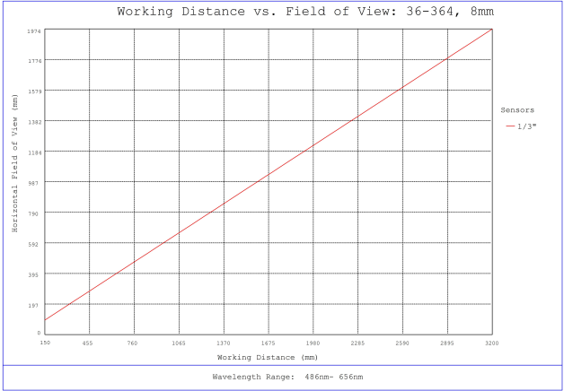
#36-364, 8.0mm FL f/2.5, Rugged Blue Series M12 Lens, Working Distance versus Field of View Plot
