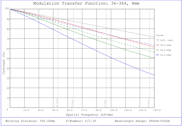
#36-364, 8.0mm FL f/2.5, Rugged Blue Series M12 Lens, Modulated Transfer Function (MTF) Plot, 350mm Working Distance, f2.5
