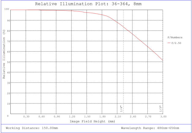
#36-364, 8.0mm FL f/2.5, Rugged Blue Series M12 Lens, Relative Illumination Plot
