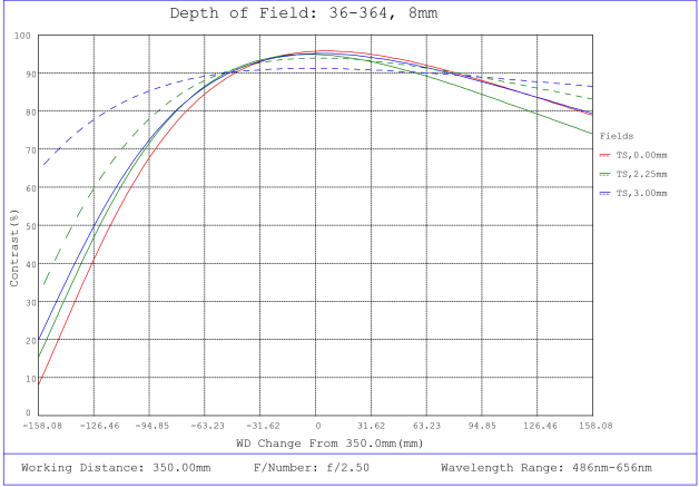
#36-364, 8.0mm FL f/2.5, Rugged Blue Series M12 Lens, Depth of Field Plot, 350mm Working Distance, f2.5
