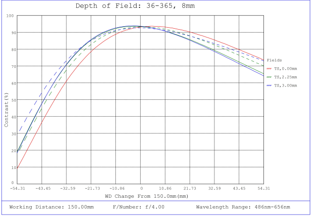
#36-365, 8.0mm FL f/4 Rugged Blue Series M12 Lens, Depth of Field Plot, 150mm Working Distance, f4
