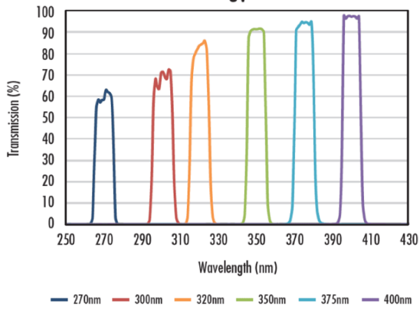
TECHSPEC® Hard Coated OD 4.0 10nm Bandpass Filters VIS
