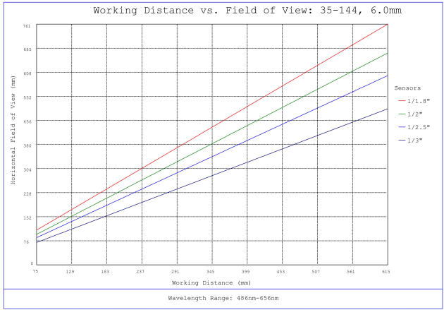
#35-144, 6mm, f/8 Cr Series Fixed Focal Length Lens, Working Distance versus Field of View Plot
