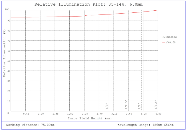
#35-144, 6mm, f/8 Cr Series Fixed Focal Length Lens, Relative Illumination Plot
