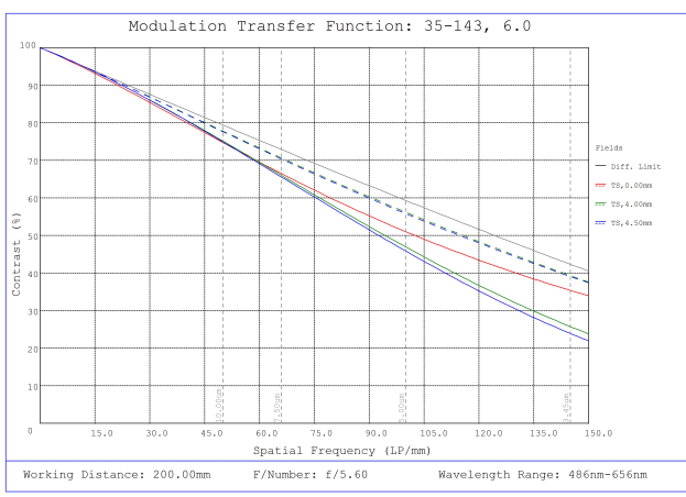
#35-143, 6mm, f/5.6 Cr Series Fixed Focal Length Lens, Modulated Transfer Function (MTF) Plot, 200mm Working Distance, f5.6
