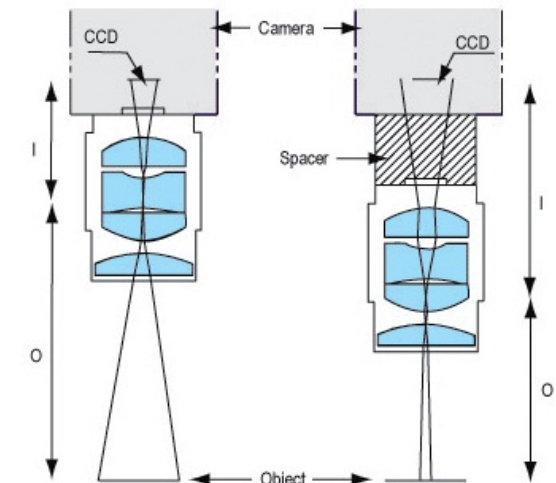
Using C-Mount Spacers in Electronic Imaging
