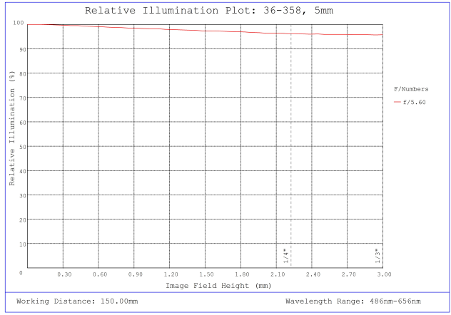
#36-358, 5mm FL f/5.6, Rugged Blue Series M12 Lens, Relative Illumination Plot
