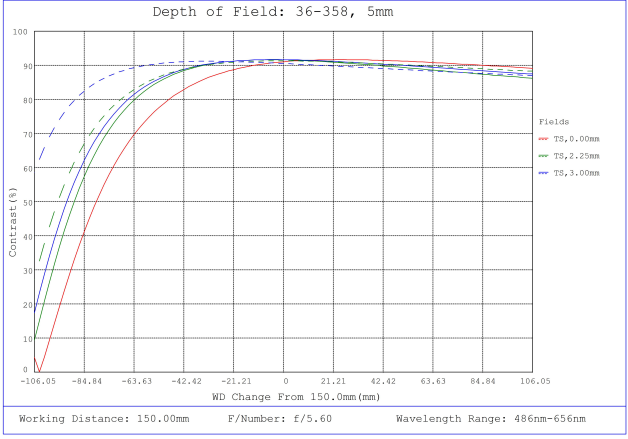
#36-358, 5mm FL f/5.6, Rugged Blue Series M12 Lens, Depth of Field Plot, 150mm Working Distance, f5.6
