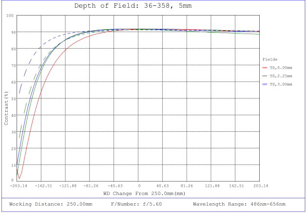
#36-358, 5mm FL f/5.6, Rugged Blue Series M12 Lens, Depth of Field Plot, 250mm Working Distance, f5.6
