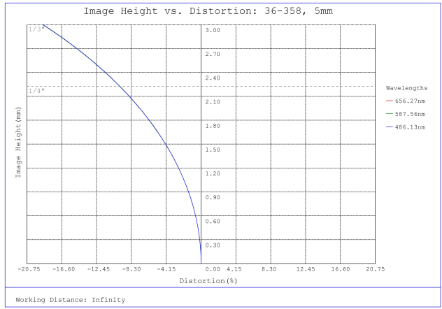
#36-358, 5mm FL f/5.6, Rugged Blue Series M12 Lens, Distortion Plot
