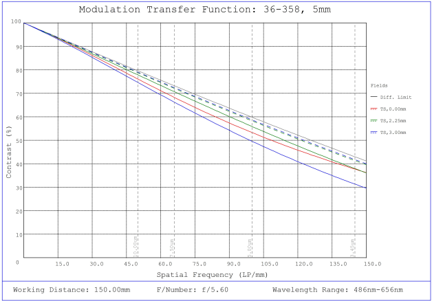
#36-358, 5mm FL f/5.6, Rugged Blue Series M12 Lens, Modulated Transfer Function (MTF) Plot, 150mm Working Distance, f5.6
