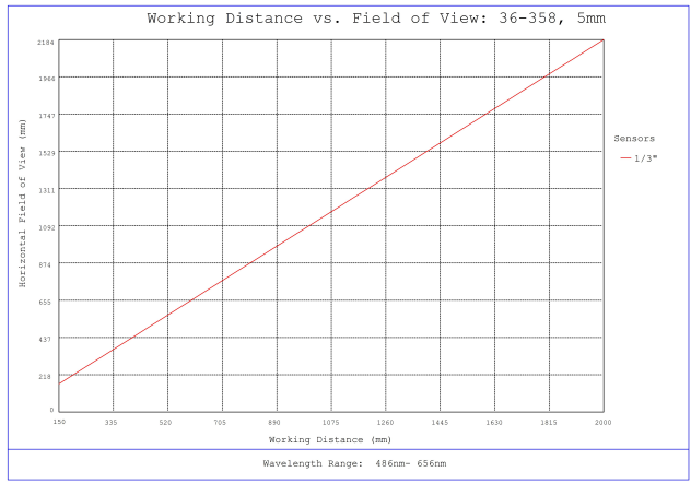
#36-358, 5mm FL f/5.6, Rugged Blue Series M12 Lens, Working Distance versus Field of View Plot
