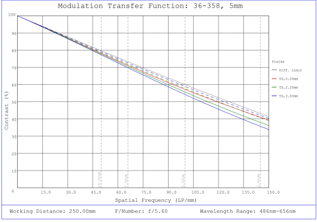
#36-358, 5mm FL f/5.6, Rugged Blue Series M12 Lens, Modulated Transfer Function (MTF) Plot, 250mm Working Distance, f5.6
