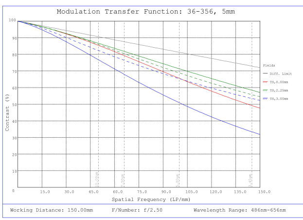
#36-356, 5mm FL f/2.5, Rugged Blue Series M12 Lens, Modulated Transfer Function (MTF) Plot, 150mm Working Distance, f2.5
