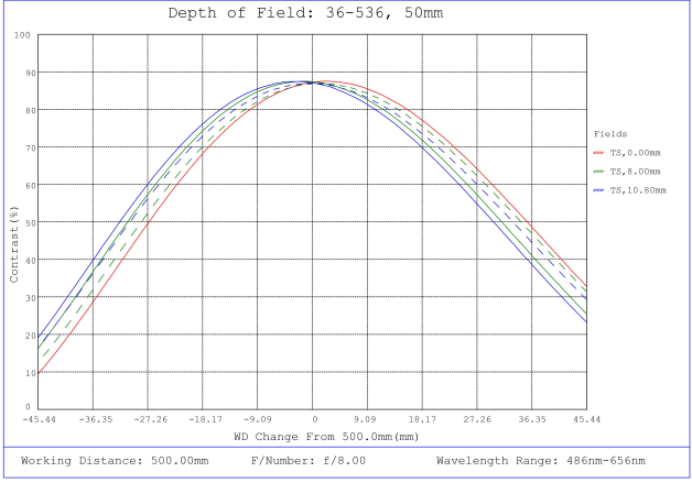
#36-536, 50mm f/8.0, HPr Series Fixed Focal Length Lens, Depth of Field Plot, 500mm Working Distance, f8
