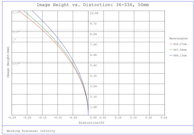
#36-536, 50mm f/8.0, HPr Series Fixed Focal Length Lens, Distortion Plot
