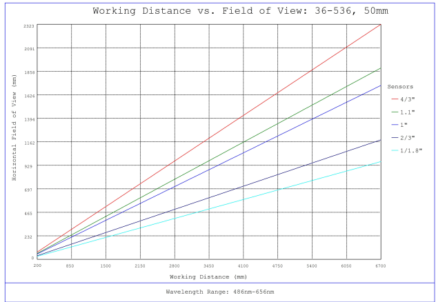
#36-536, 50mm f/8.0, HPr Series Fixed Focal Length Lens, Working Distance versus Field of View Plot
