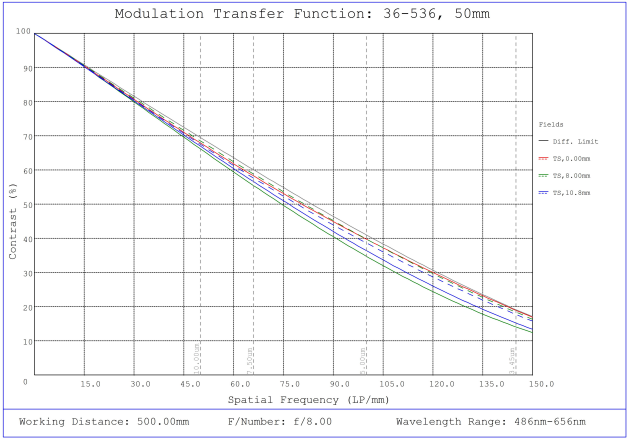
#36-536, 50mm f/8.0, HPr Series Fixed Focal Length Lens, Modulated Transfer Function (MTF) Plot, 500mm Working Distance, f8
