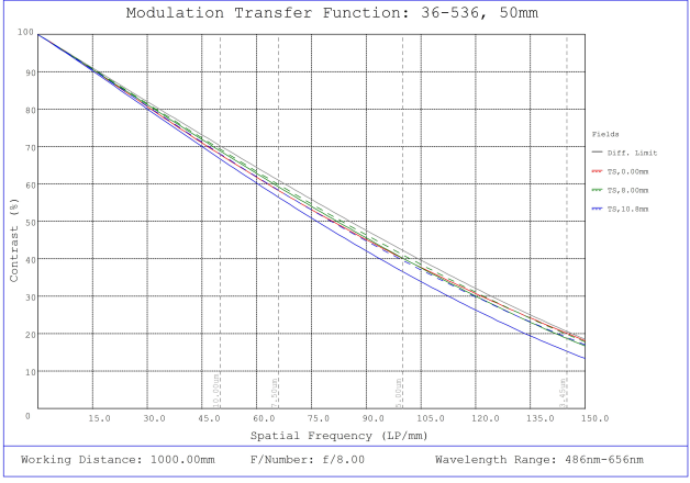
#36-536, 50mm f/8.0, HPr Series Fixed Focal Length Lens, Modulated Transfer Function (MTF) Plot, 1000mm Working Distance, f8
