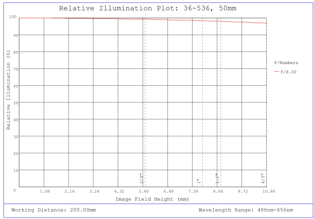
#36-536, 50mm f/8.0, HPr Series Fixed Focal Length Lens, Relative Illumination Plot
