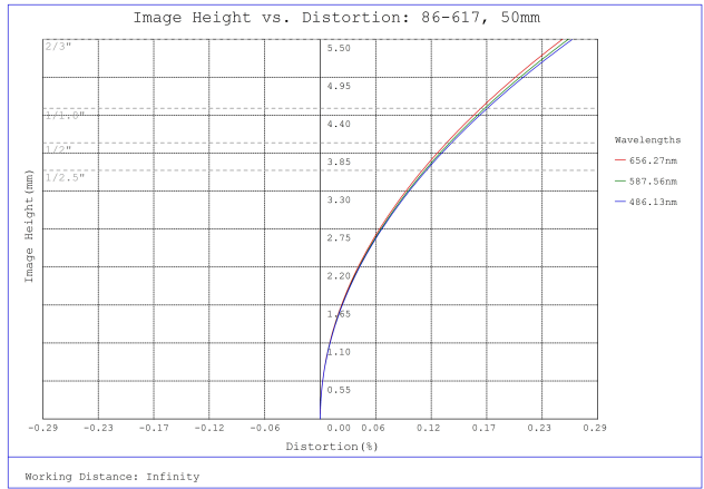
#86-617, 50mm, f/5.6 Ci Series Fixed Focal Length Lens, Distortion Plot
