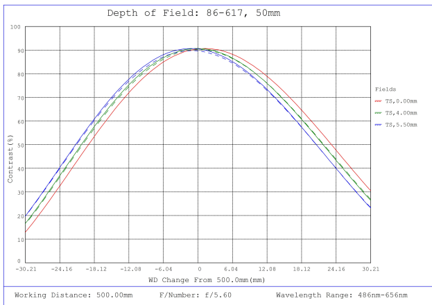
#86-617, 50mm, f/5.6 Ci Series Fixed Focal Length Lens, Depth of Field Plot, 500mm Working Distance, f5.6
