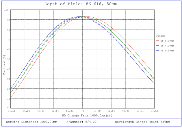
#86-616, 50mm, f/4.0 Ci Series Fixed Focal Length Lens, Depth of Field Plot, 1000mm Working Distance, f4
