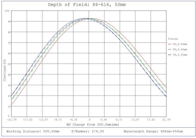
#86-616, 50mm, f/4.0 Ci Series Fixed Focal Length Lens, Depth of Field Plot, 500mm Working Distance, f4
