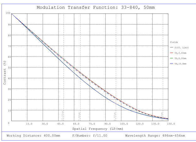
#33-840, 50mm f/11, HPI Series Fixed Focal Length Lens, Modulated Transfer Function (MTF) Plot, 400mm Working Distance, f11
