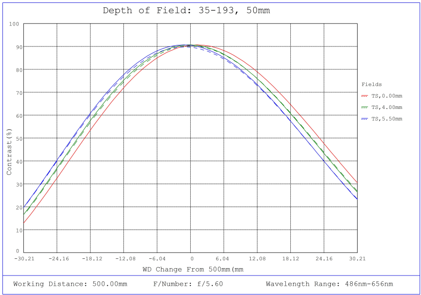
#35-193, 50mm, f/5.6 Cr Series Fixed Focal Length Lens, Depth of Field Plot, 500mm Working Distance, f5.6
