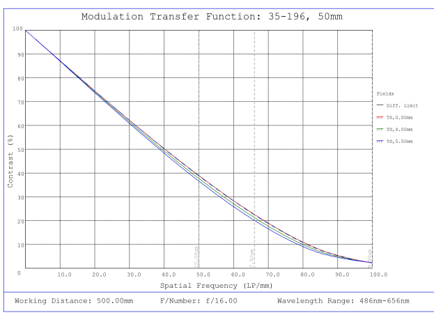
#35-196, 50mm, f/16 Cr Series Fixed Focal Length Lens, Modulated Transfer Function (MTF) Plot, 500mm Working Distance, f16
