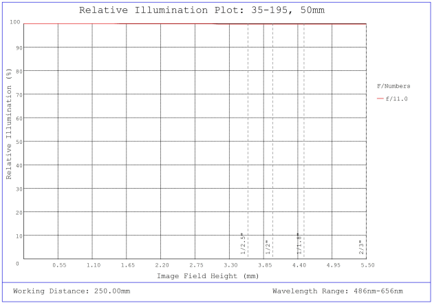
#35-195, 50mm, f/11 Cr Series Fixed Focal Length Lens, Relative Illumination Plot
