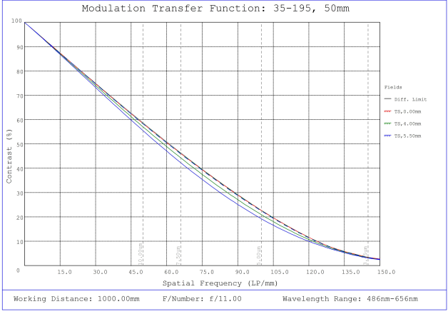
#35-195, 50mm, f/11 Cr Series Fixed Focal Length Lens, Modulated Transfer Function (MTF) Plot, 1000mm Working Distance, f11
