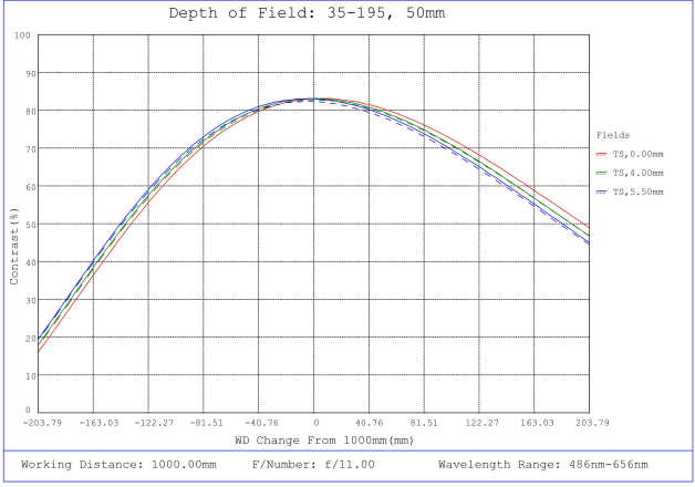
#35-195, 50mm, f/11 Cr Series Fixed Focal Length Lens, Depth of Field Plot, 1000mm Working Distance, f11
