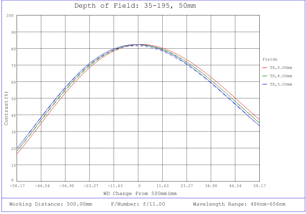
#35-195, 50mm, f/11 Cr Series Fixed Focal Length Lens, Depth of Field Plot, 500mm Working Distance, f11
