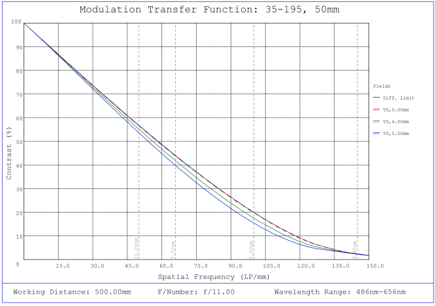
#35-195, 50mm, f/11 Cr Series Fixed Focal Length Lens, Modulated Transfer Function (MTF) Plot, 500mm Working Distance, f11
