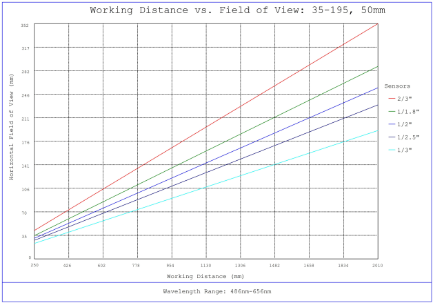
#35-195, 50mm, f/11 Cr Series Fixed Focal Length Lens, Working Distance versus Field of View Plot
