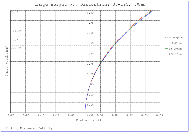
#35-195, 50mm, f/11 Cr Series Fixed Focal Length Lens, Distortion Plot
