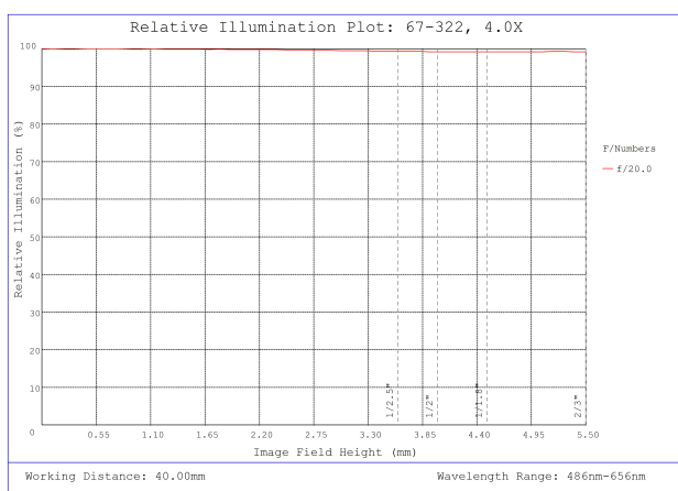
#67-322, 4X, 40mm WD, In-Line CompactTL™ Telecentric Lens, Relative Illumination Plot
