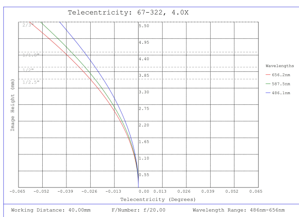
#67-322, 4X, 40mm WD, In-Line CompactTL™ Telecentric Lens, Telecentricity Plot
