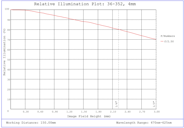
#36-352, 4mm FL f/2.5, Rugged Blue Series M12 Lens, Relative Illumination Plot
