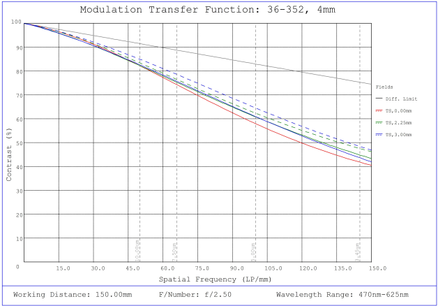
#36-352, 4mm FL f/2.5, Rugged Blue Series M12 Lens, Modulated Transfer Function (MTF) Plot, 150mm Working Distance, f2.5
