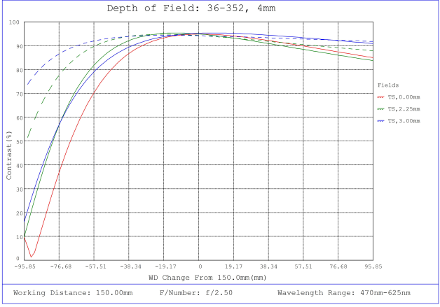
#36-352, 4mm FL f/2.5, Rugged Blue Series M12 Lens, Depth of Field Plot, 150mm Working Distance, f2.5
