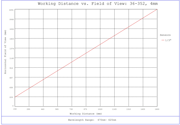
#36-352, 4mm FL f/2.5, Rugged Blue Series M12 Lens, Working Distance versus Field of View Plot
