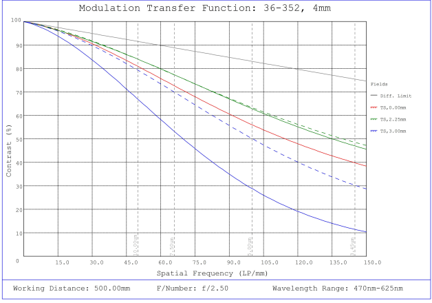
#36-352, 4mm FL f/2.5, Rugged Blue Series M12 Lens, Modulated Transfer Function (MTF) Plot, 500mm Working Distance, f2.5
