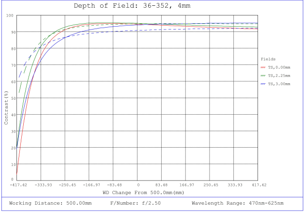
#36-352, 4mm FL f/2.5, Rugged Blue Series M12 Lens, Depth of Field Plot, 500mm Working Distance, f2.5
