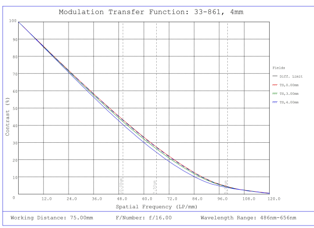
#33-861, 4mm, f/16 UCI Series Fixed Focal Length Lens, Modulated Transfer Function (MTF) Plot, 75mm Working Distance, f16
