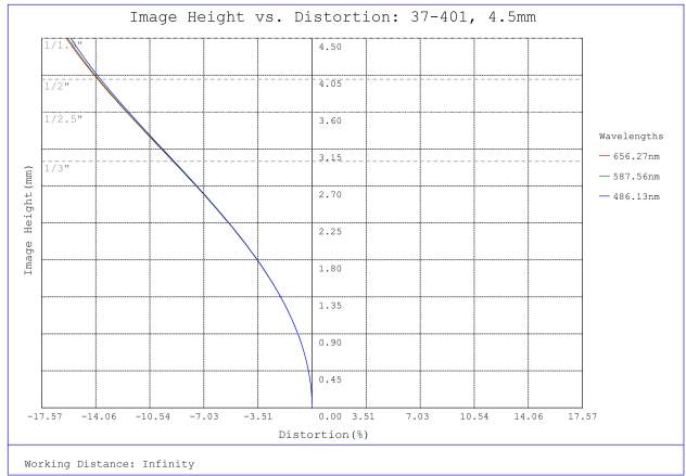
#37-401, 4.5mm, f/5.6 Cr Series Fixed Focal Length Lens, Distortion Plot
