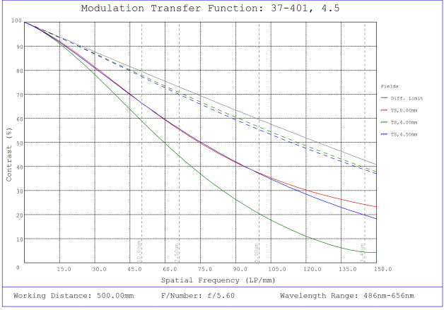
#37-401, 4.5mm, f/5.6 Cr Series Fixed Focal Length Lens, Modulated Transfer Function (MTF) Plot, 500mm Working Distance, f5.6
