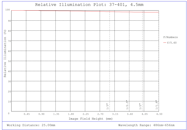
#37-401, 4.5mm, f/5.6 Cr Series Fixed Focal Length Lens, Relative Illumination Plot
