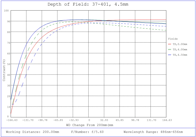
#37-401, 4.5mm, f/5.6 Cr Series Fixed Focal Length Lens, Depth of Field Plot, 200mm Working Distance, f5.6
