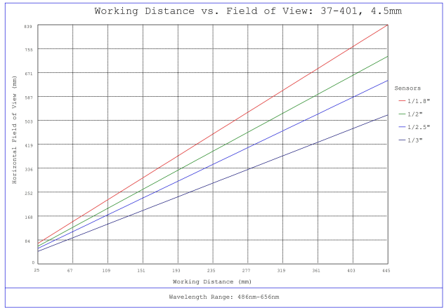
#37-401, 4.5mm, f/5.6 Cr Series Fixed Focal Length Lens, Working Distance versus Field of View Plot
