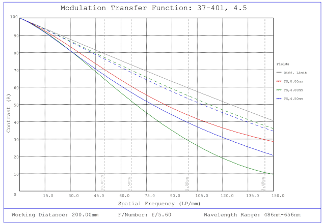
#37-401, 4.5mm, f/5.6 Cr Series Fixed Focal Length Lens, Modulated Transfer Function (MTF) Plot, 200mm Working Distance, f5.6
