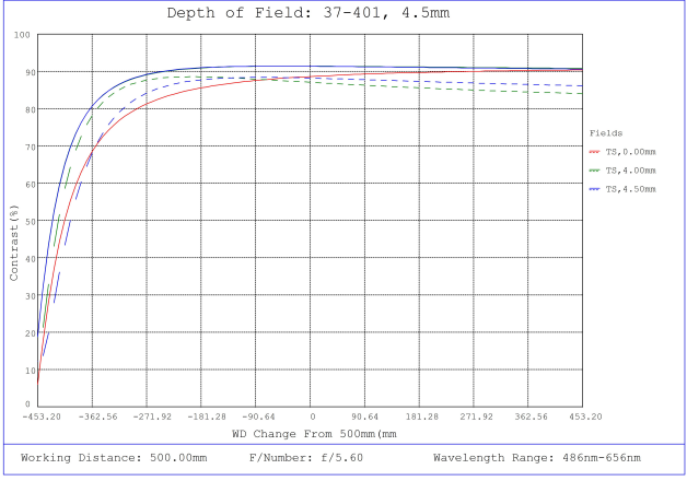
#37-401, 4.5mm, f/5.6 Cr Series Fixed Focal Length Lens, Depth of Field Plot, 500mm Working Distance, f5.6
