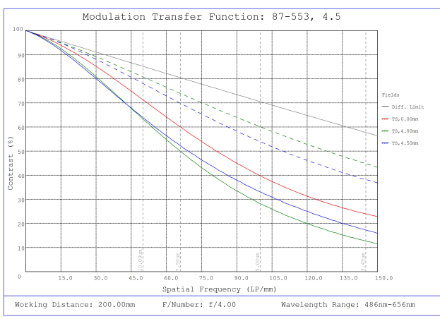
#87-553, 4.5mm, f/4 Ci Series Fixed Focal Length Lens, Modulated Transfer Function (MTF) Plot, 200mm Working Distance, f4
