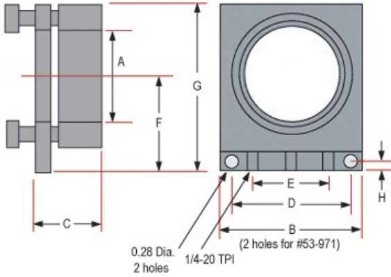
4.25" Straight Optical Cell Mount
