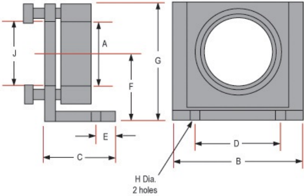
1" - 4.25" Angled Optical Cell Mounts
