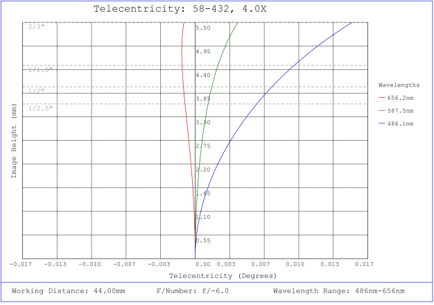
#58-432, 4.0X SilverTL™ Telecentric Lens, Telecentricity Plot
