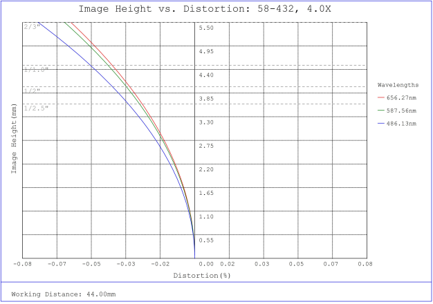
#58-432, 4.0X SilverTL™ Telecentric Lens, Distortion Plot
