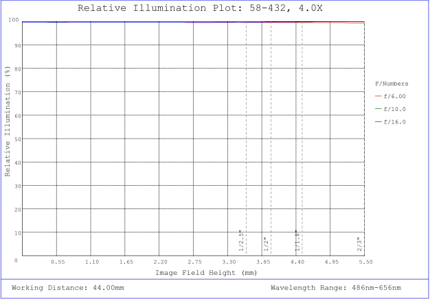
#58-432, 4.0X SilverTL™ Telecentric Lens, Relative Illumination Plot
