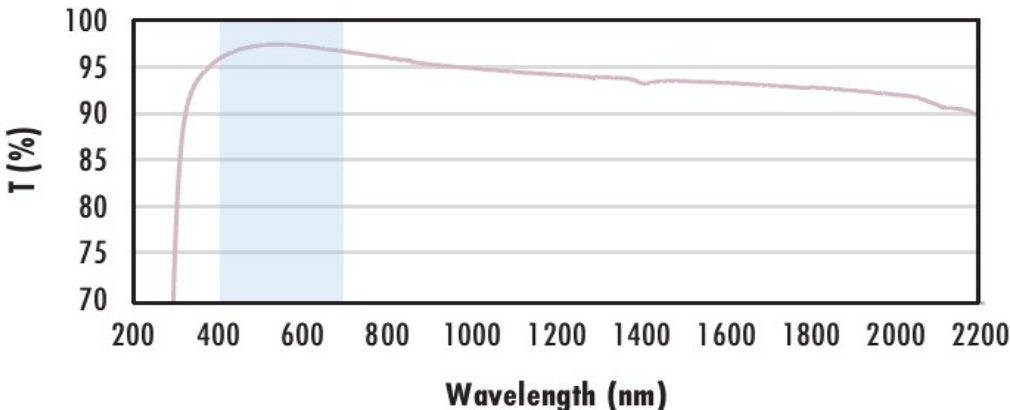
N-BK7 with MgF 2 Coating Typical Transmission
