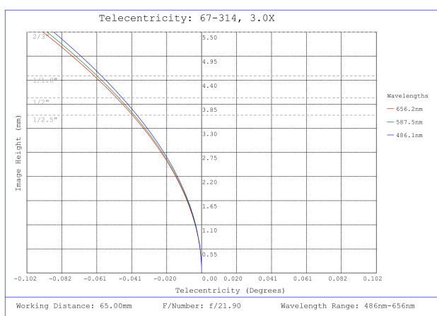
#67-314, 3X, 65mm WD, In-Line CompactTL™ Telecentric Lens, Telecentricity Plot
