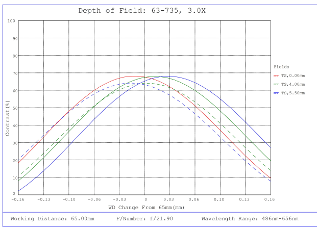
#63-735, 3X, 65mm WD CompactTL™ Telecentric Lens, Depth of Field Plot, 65mm Working Distance, f21.9
