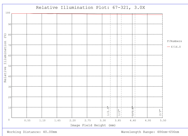
#67-321, 3X, 40mm WD, In-Line CompactTL™ Telecentric Lens, Relative Illumination Plot
