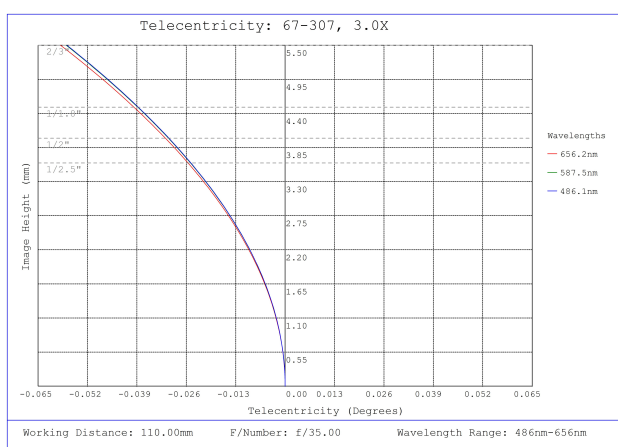
#67-307, 3X, 110mm WD, In-Line CompactTL™ Telecentric Lens, Telecentricity Plot
