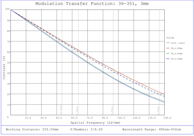
#36-351, 3mm FL f/8, Rugged Blue Series M12 Lens, Modulated Transfer Function (MTF) Plot, 250mm Working Distance, f8
