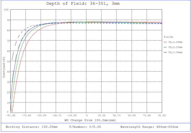
#36-351, 3mm FL f/8, Rugged Blue Series M12 Lens, Depth of Field Plot, 100mm Working Distance, f8
