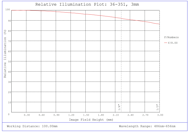
#36-351, 3mm FL f/8, Rugged Blue Series M12 Lens, Relative Illumination Plot
