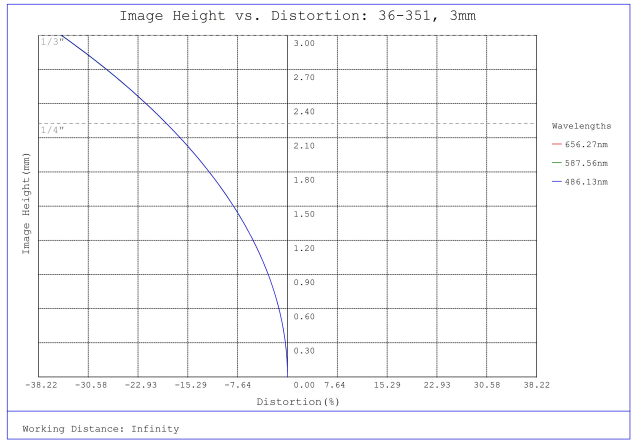
#36-351, 3mm FL f/8, Rugged Blue Series M12 Lens, Distortion Plot
