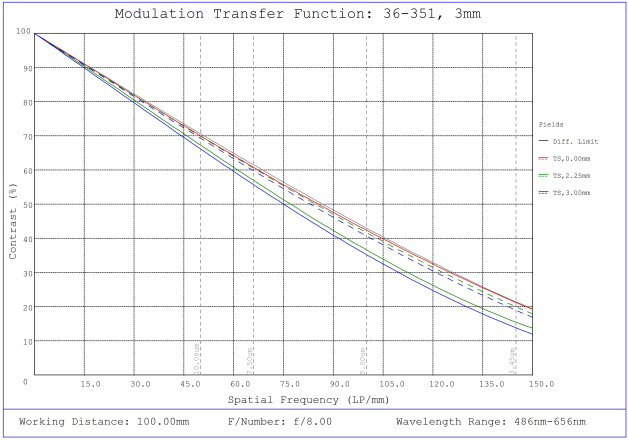
#36-351, 3mm FL f/8, Rugged Blue Series M12 Lens, Modulated Transfer Function (MTF) Plot, 100mm Working Distance, f8
