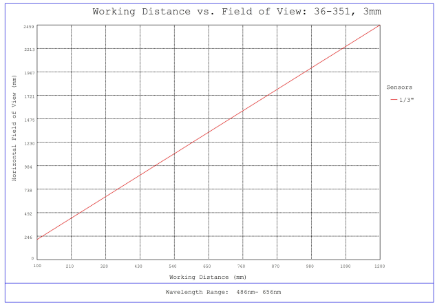
#36-351, 3mm FL f/8, Rugged Blue Series M12 Lens, Working Distance versus Field of View Plot
