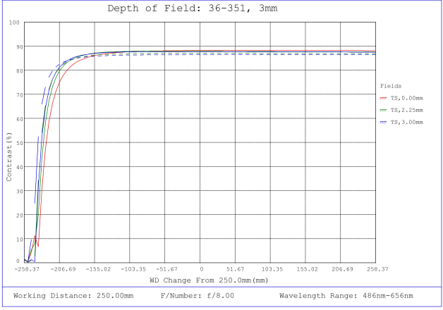
#36-351, 3mm FL f/8, Rugged Blue Series M12 Lens, Depth of Field Plot, 250mm Working Distance, f8
