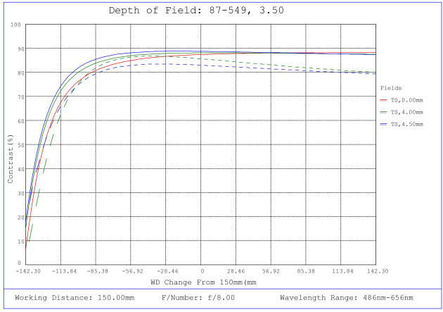
#87-549, 3.5mm, f/8 Ci Series Fixed Focal Length Lens, Depth of Field Plot, 150mm Working Distance, f8
