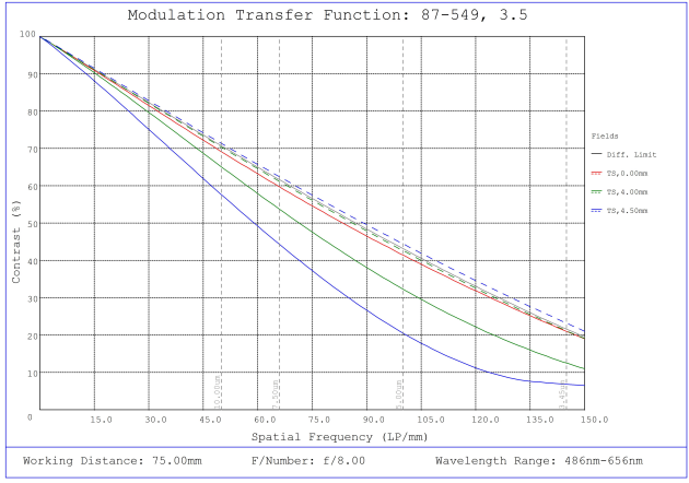
#87-549, 3.5mm, f/8 Ci Series Fixed Focal Length Lens, Modulated Transfer Function (MTF) Plot, 75mm Working Distance, f8
