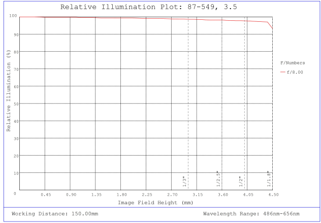
#87-549, 3.5mm, f/8 Ci Series Fixed Focal Length Lens, Relative Illumination Plot
