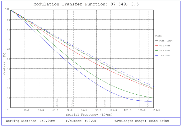
#87-549, 3.5mm, f/8 Ci Series Fixed Focal Length Lens, Modulated Transfer Function (MTF) Plot, 150mm Working Distance, f8
