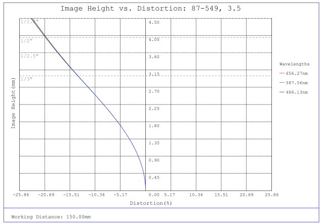
#87-549, 3.5mm, f/8 Ci Series Fixed Focal Length Lens, Distortion Plot
