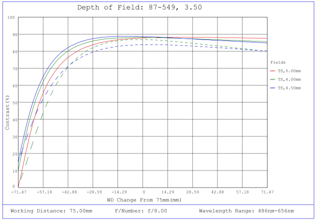
#87-549, 3.5mm, f/8 Ci Series Fixed Focal Length Lens, Depth of Field Plot, 75mm Working Distance, f8
