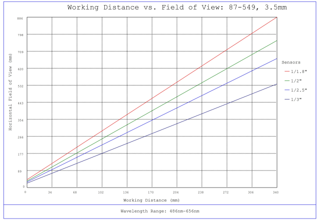
#87-549, 3.5mm, f/8 Ci Series Fixed Focal Length Lens, Working Distance versus Field of View Plot
