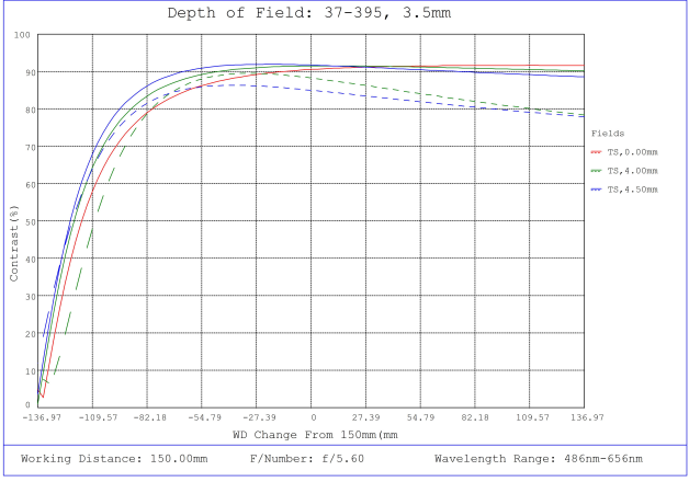
#37-395, 3.5mm, f/5.6 Cr Series Fixed Focal Length Lens, Depth of Field Plot, 150mm Working Distance, f5.6
