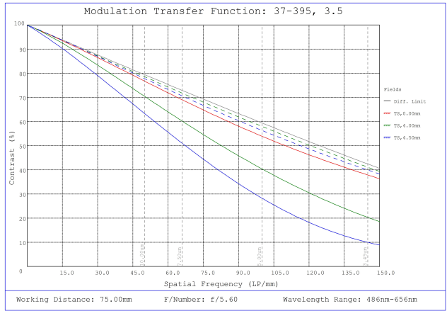
#37-395, 3.5mm, f/5.6 Cr Series Fixed Focal Length Lens, Modulated Transfer Function (MTF) Plot, 75mm Working Distance, f5.6
