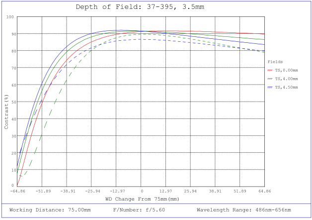
#37-395, 3.5mm, f/5.6 Cr Series Fixed Focal Length Lens, Depth of Field Plot, 75mm Working Distance, f5.6
