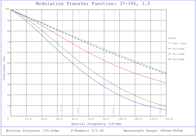
#37-395, 3.5mm, f/5.6 Cr Series Fixed Focal Length Lens, Modulated Transfer Function (MTF) Plot, 150mm Working Distance, f5.6
