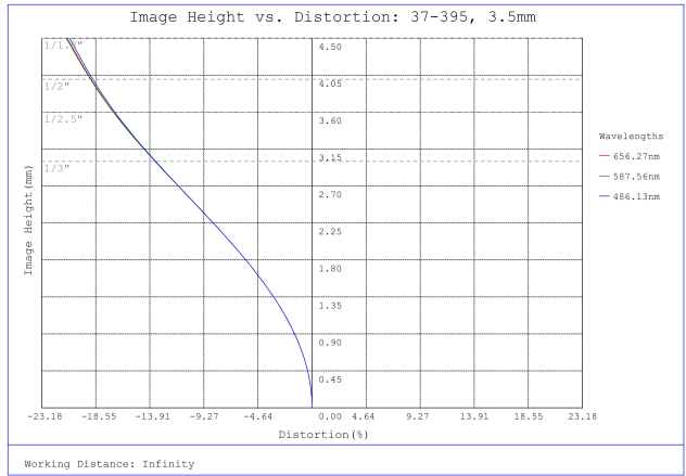
#37-395, 3.5mm, f/5.6 Cr Series Fixed Focal Length Lens, Distortion Plot
