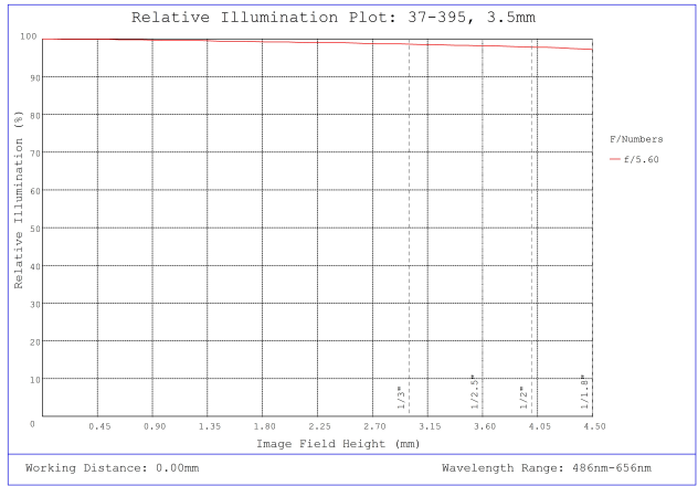
#37-395, 3.5mm, f/5.6 Cr Series Fixed Focal Length Lens, Relative Illumination Plot
