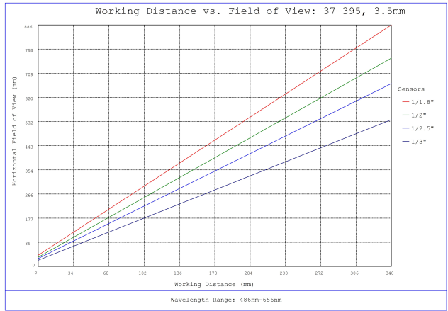
#37-395, 3.5mm, f/5.6 Cr Series Fixed Focal Length Lens, Working Distance versus Field of View Plot
