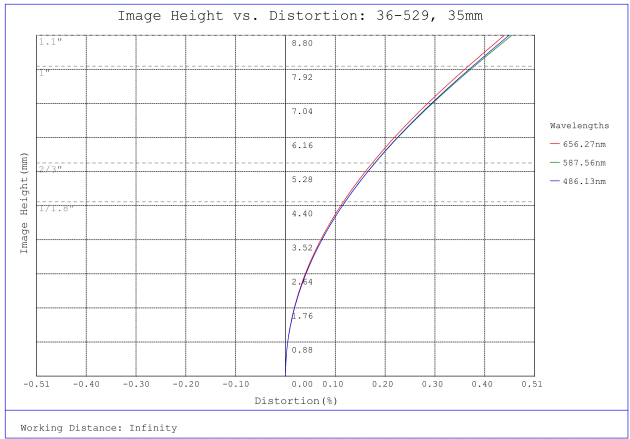
#36-529, 35mm f/5.6, HPr Series Fixed Focal Length Lens, Distortion Plot
