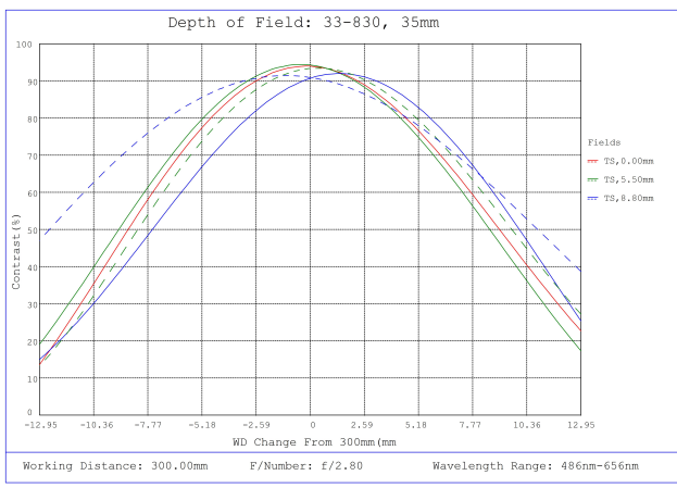
#33-830, 35mm f/2.8, HPI Series Fixed Focal Length Lens, Depth of Field Plot, 300mm Working Distance, f2.8
