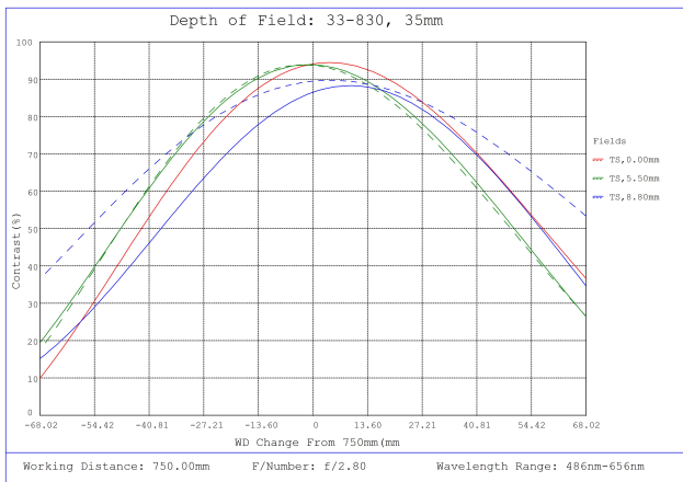
#33-830, 35mm f/2.8, HPI Series Fixed Focal Length Lens, Depth of Field Plot, 750mm Working Distance, f2.8
