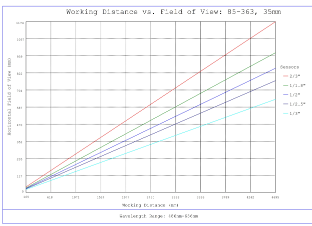
#85-363, 35mm, f/1.8 Ci Series Fixed Focal Length Lens, Working Distance versus Field of View Plot
