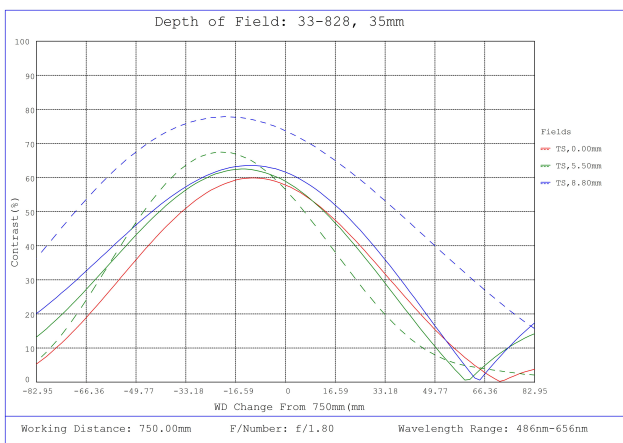
#33-828, 35mm f/1.8, HPI Series Fixed Focal Length Lens, Depth of Field Plot, 750mm Working Distance, f1.8
