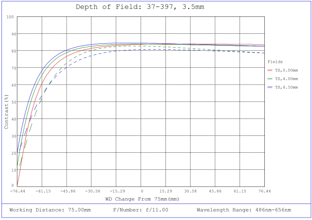
#37-397, 3.5mm, f/11 Cr Series Fixed Focal Length Lens, Depth of Field Plot, 75mm Working Distance, f11
