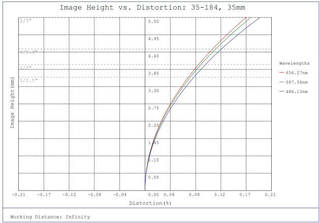
#35-184, 35mm, f/4.0 Cr Series Fixed Focal Length Lens, Distortion Plot
