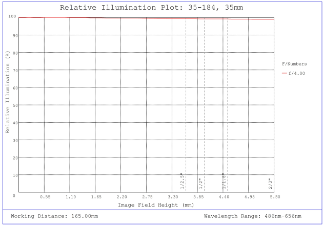
#35-184, 35mm, f/4.0 Cr Series Fixed Focal Length Lens, Relative Illumination Plot
