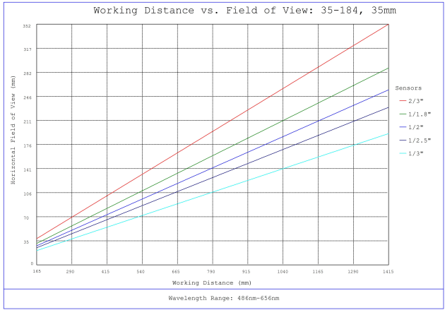
#35-184, 35mm, f/4.0 Cr Series Fixed Focal Length Lens, Working Distance versus Field of View Plot
