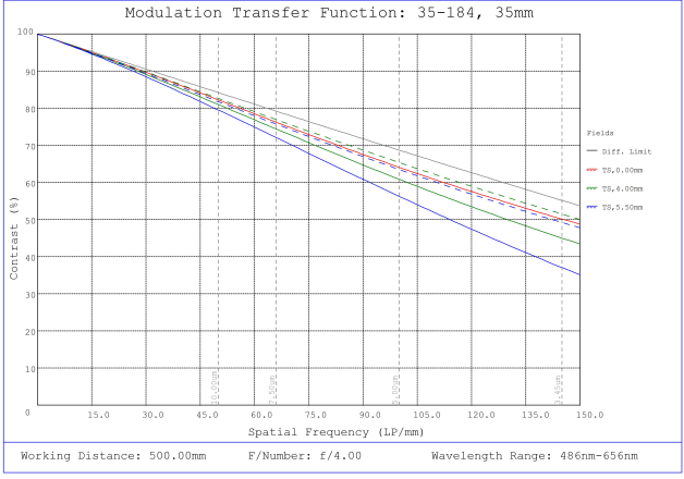
#35-184, 35mm, f/4.0 Cr Series Fixed Focal Length Lens, Modulated Transfer Function (MTF) Plot, 500mm Working Distance, f4
