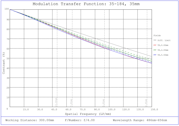
#35-184, 35mm, f/4.0 Cr Series Fixed Focal Length Lens, Modulated Transfer Function (MTF) Plot, 300mm Working Distance, f4
