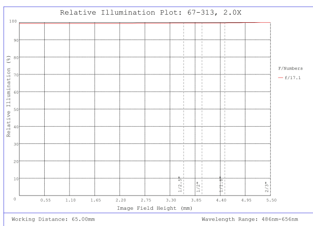
#67-313, 2X, 65mm WD, In-Line CompactTL™ Telecentric Lens, Relative Illumination Plot
