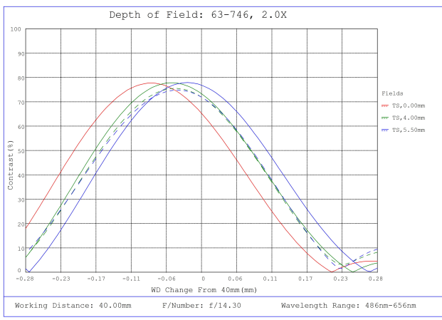
#63-746, 2X, 40mm WD CompactTL™ Telecentric Lens , Depth of Field Plot, 40mm Working Distance, f14.3
