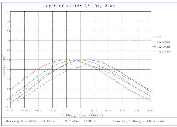
#33-101, 2X, 300mm WD CompactTL™ Telecentric Lens, Depth of Field Plot, 300mm Working Distance, f28.5
